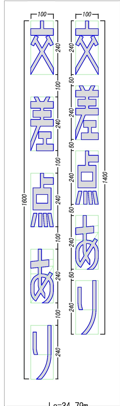
Le=34.79m Lp=41.5m
